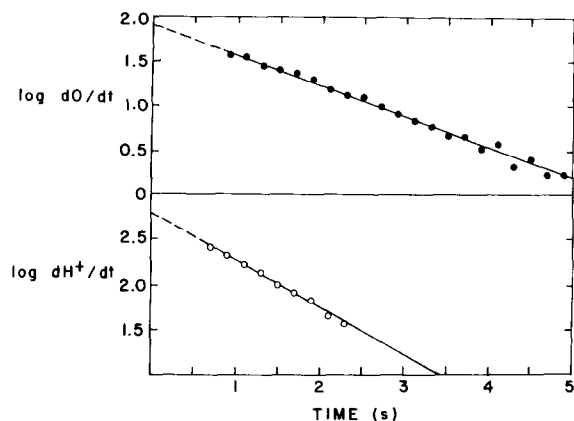
Fig. 1. H^+ and O_2 electrode data obtained when succinate oxidation was initiated by photoactivation of CO-inhibited electron flow through cytochrome c oxidase. The basic medium of 50 mM KCl, 200 mM sucrose, 1.5 mM K^+ -Hepes, pH 7.05 (6.0 ml, t = 25^\circ\text{C} ) in a glass reaction vessel was made nearly anaerobic with a stream of N_2 and 100% CO then passed over the surface at a rate of 80 ml/min. Rotenone (2 \mu\text{M} ) and succinate (5.0 mM) were added in microliter volumes followed by rat liver mitochondria (18 mg protein) in 0.3 M sucrose. O_2 admitted during the additions was depleted by illumination of the suspension until the O_2 trace was essentially zero; 18 \mu\text{g} oligomycin, 90 \mu\text{g} N -ethylmaleimide and 2.2 \mu\text{g} valinomycin were then added. Illumination was stopped and the suspension incubated in the dark for 20 min under CO. A known amount of O_2 (45.0 nmol O ) in air-saturated medium was added in the dark; this addition also served for calibration of the O_2 electrode. After further dark incubation (30 s), which established the zero time baselines, the shutter was opened to initiate electron flow. The pH electrode was calibrated at the end of the experiment with 400 nmol HCl. The signals for both electrodes were accessed directly into the computer at 10-ms intervals. Data from 0.8 to 5 s for the oxygen electrode and from 0.8 to 3 s for the pH electrode were fitted to the rate expression S = Ae^{-kt} + A_\infty for evaluation of the parameters A , k , and A_\infty . The raw data for the rates ( X ) as well as the continuous plots obtained from the best-fit parameters are shown in semi-log form for the O_2 electrode (upper panel) and the H^+ electrode (lower panel). The extrapolated H^+/O ratio at true zero time was 7.83.
