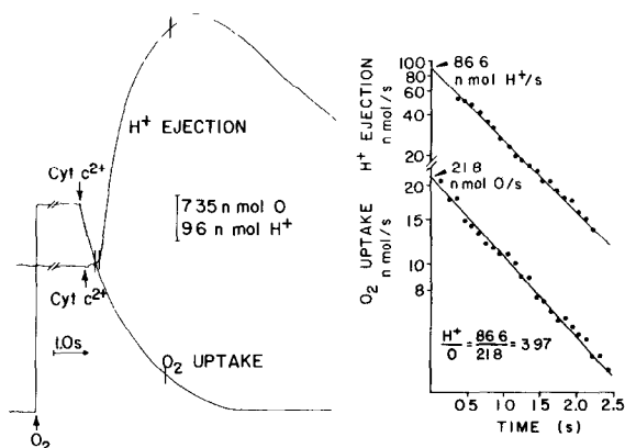
Fig. 2. The H^+/O ratio for the cytochrome oxidase reaction initiated by ferrocytochrome c . The reaction system (1.50 ml, t = 10^\circ\text{C} ) consisted of 50 mM KCl, 200 mM sucrose, 3.0 mM K^+ -Hepes pH 7.10, antimycin A (0.1 nmol/mg), N -ethylmaleimide (40 nmol/mg), valinomycin (300 ng/mg), about 10 \mu\text{M} O_2 , and rat liver mitochondria (2.5 mg protein). After stabilization of the electrode traces 180 nmol cyt. c^{2+} was injected to initiate electron flow and the O_2 uptake and H^+ ejection recorded as shown in the reaction traces. Points were taken at 0.1-s intervals from the unsmoothed traces between the vertical bars, digitized, and shown in the form of Guggenheim plots (right), fitted by a weighted regression analysis. The time at which mixing was complete in this experiment (i.e. zero time) was approximated to be 0.1 s after start of the injection of cyt. c^{2+} . This approximation was made possible because the O_2 electrode employed had a 90% response time of < 0.1 s, as can be seen from the rapid response of the O_2 trace to the injection of O_2 . However, since the H^+ electrode had a much longer 90% response time ( \sim 0.6 s), only the data taken from comparable points of the traces beginning at 0.5 s were used to extrapolate the initial H^+/O ratio, which was 3.97 at 0.1 s.
